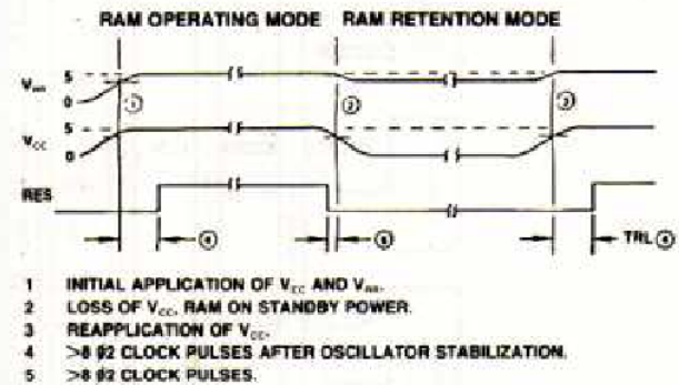
FIGURE 3-2. Data Retention Timing
