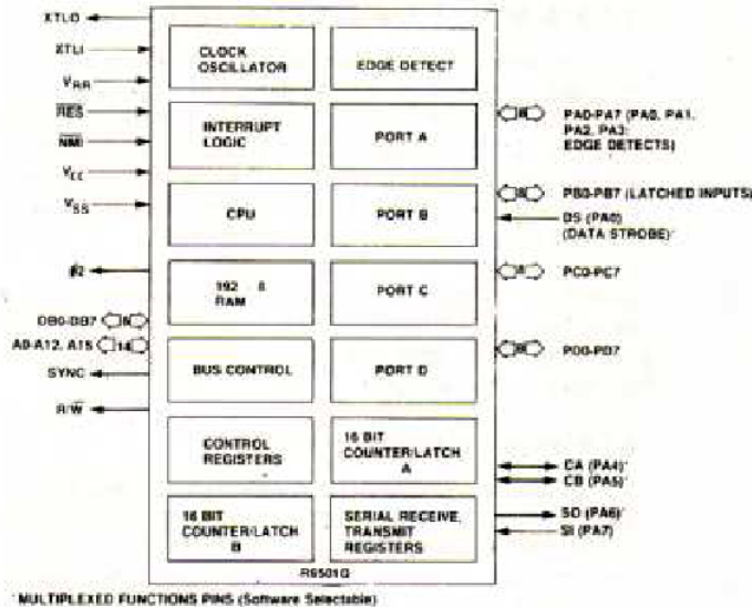
FIGURE 2-2. Interface Diagram
