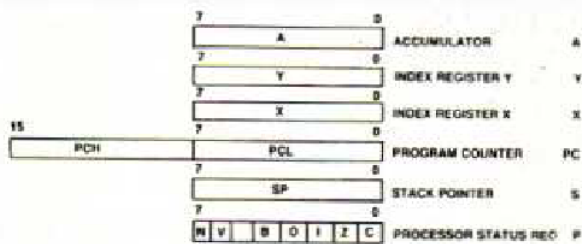
CPU Registers
