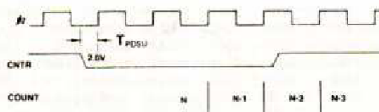
FIGURE 6-3. Pulse Width Measurement
