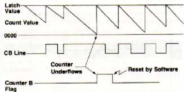
FIGURE 6-4. Counter B, Retriggerable Interval Timer Mode
