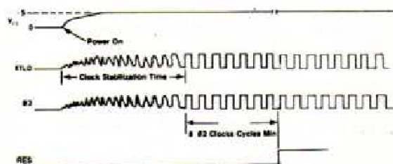
FIGURE 7-1. Power Turn-On Timing Detail
