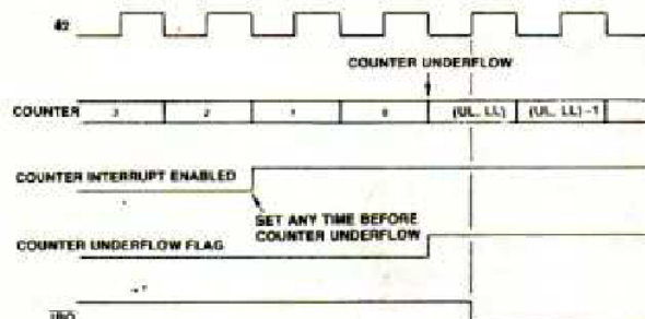
FIGURE 6-1. Interval Timer Timing Diagram
