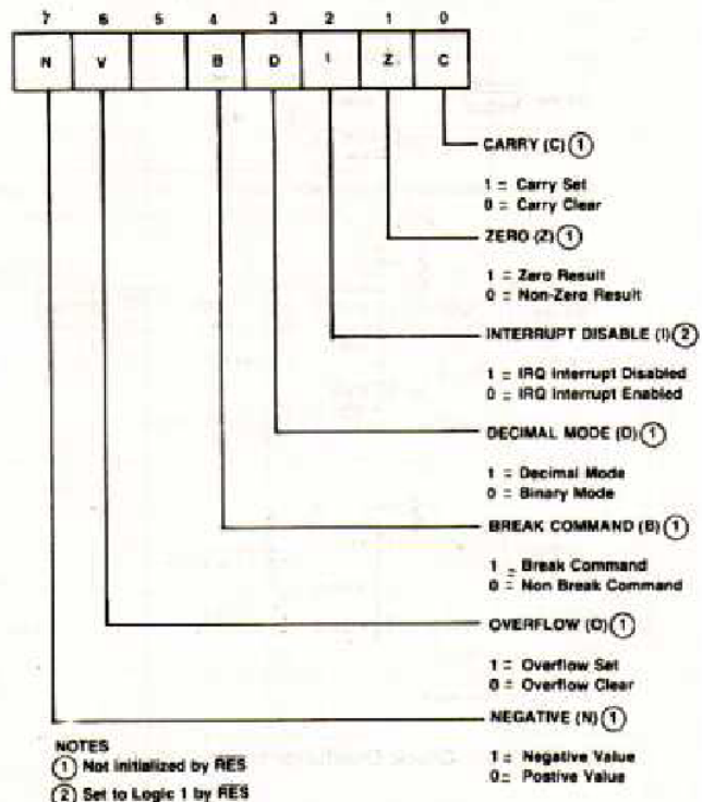
FIGURE 3-7. Processor Status Register
