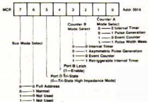
Mode Control Register
