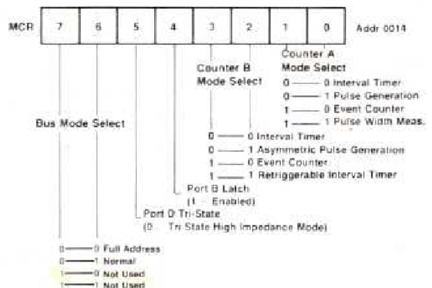
FIGURE 3-5. Mode Control Register
