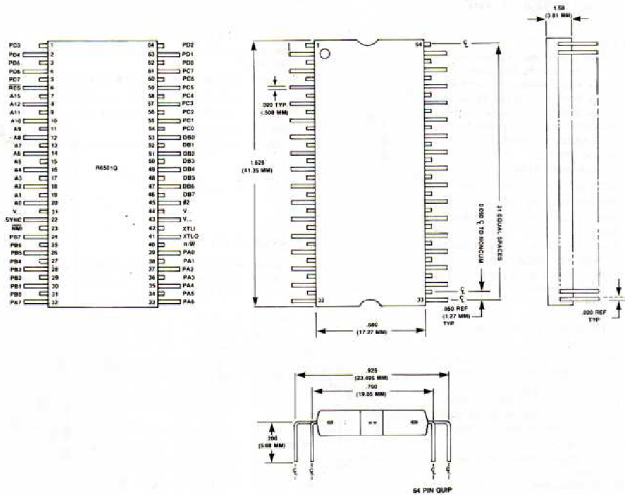
FIGURE 2-1. Mechanical Outline & Pin Out Configuration
