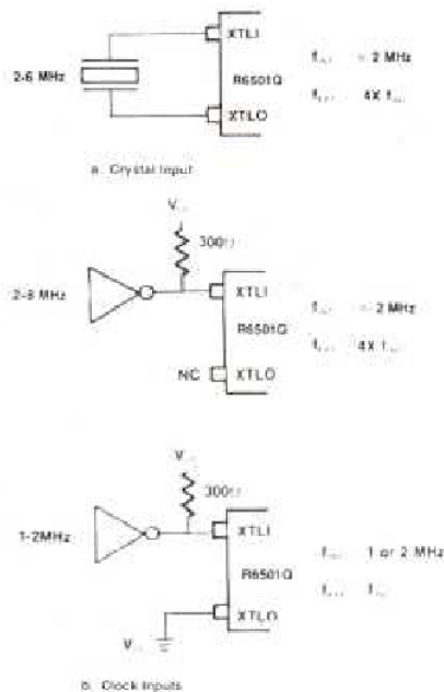
FIGURE 3-3. Clock Oscillator Input Options
