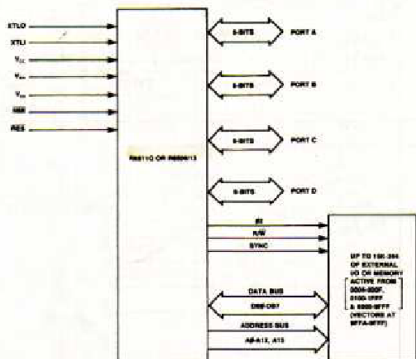
FIGURE 4-1b. Normal Bus Mode
