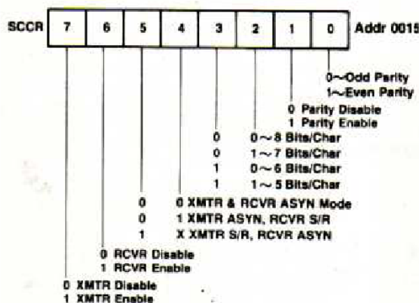
FIGURE 5-1. Serial Communication Control Register
